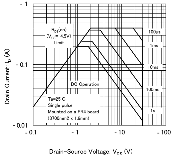
(8) Area of Safe Operation
