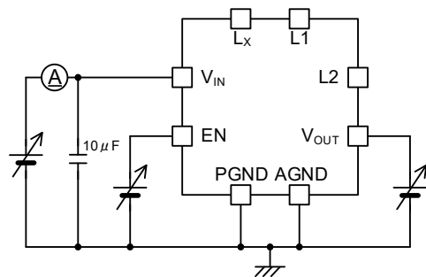
<Circuit No.2>
