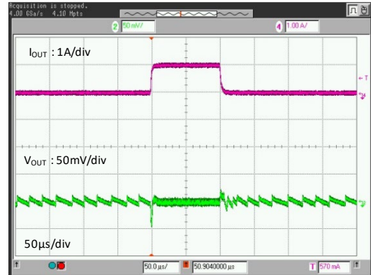
XCL238, V_{OUT(T)}=1.8V
