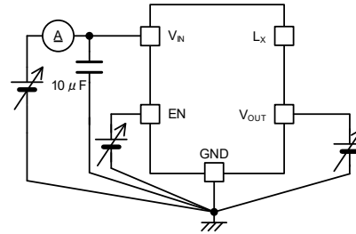
< Circuit No.2 >
