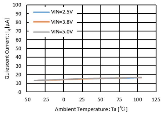
XC9288, f_{OSC} = 3MHz
