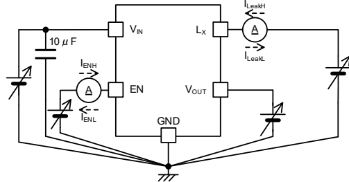
< Circuit No.5 >
