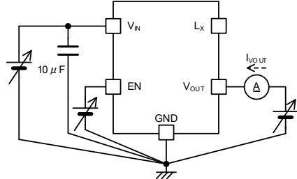
< Circuit No.7 > B Type
