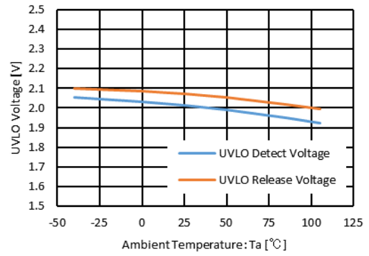
XC9288, f_{OSC} = 1.2MHz
