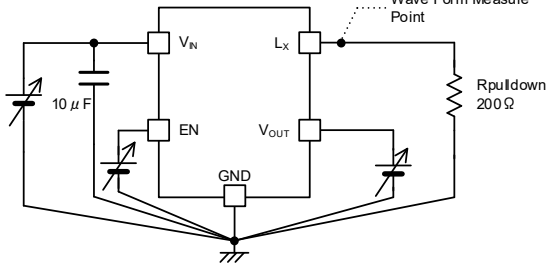
< Circuit No.3 >
