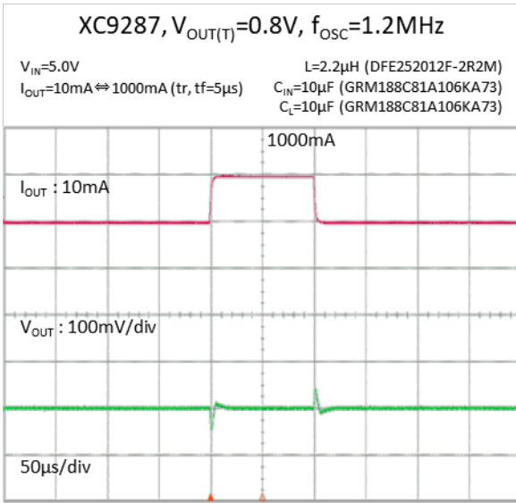
(20) Load Transient Response
