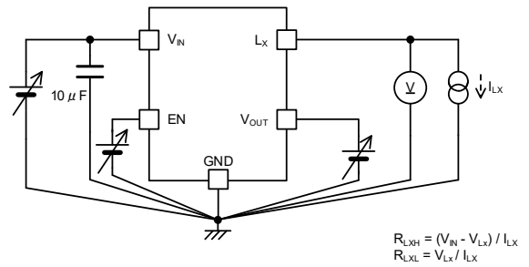
< Circuit No.6 >
