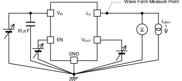
< Circuit No.6 >
