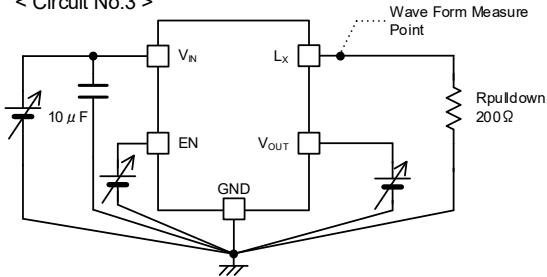
< Circuit No.3 >
