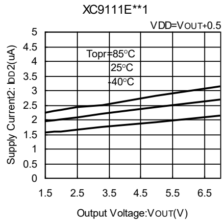
(7) No Load Input Current vs. Output Voltage
