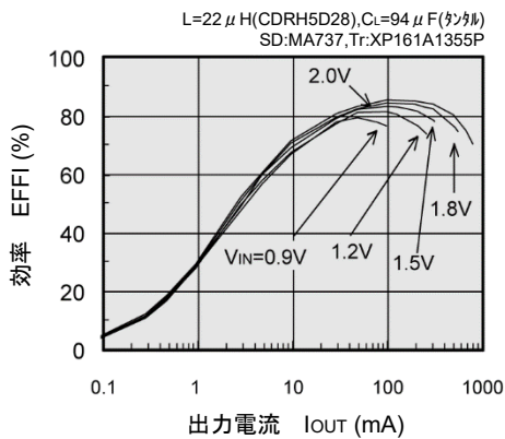
XC9103D093MR (PWM, 300kHz, 3.3V 品)
