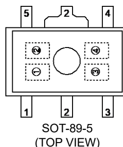
●SOT-89-5
