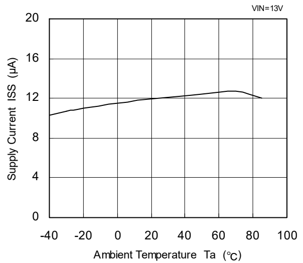
XC6202PC02(12V)
