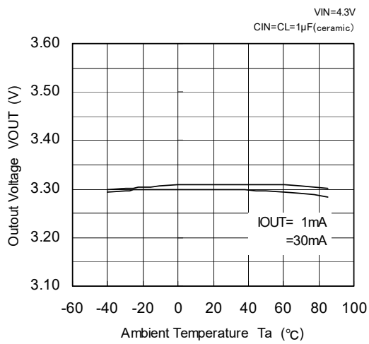
XC6202P332 (3.3V)
