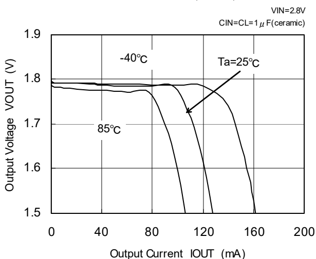
XC6202P182(1.8V)
