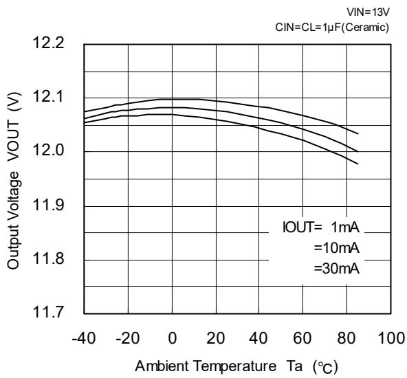
XC6202PC02(12V)
