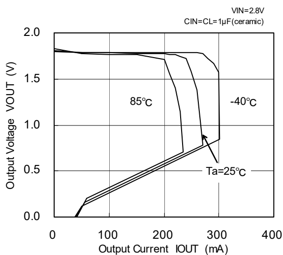
XC6202P182(1.8V)
