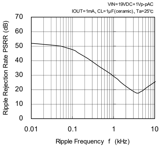
XC6202PJ02(18V)
