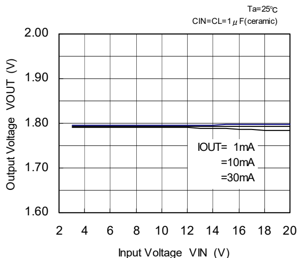
XC6202P182(1.8V)
