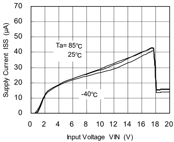
XC6202PJ02 (18V)
