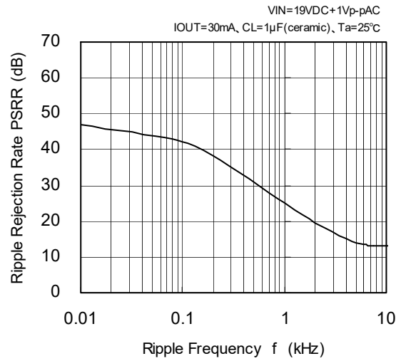
XC6202PJ02(18V)
