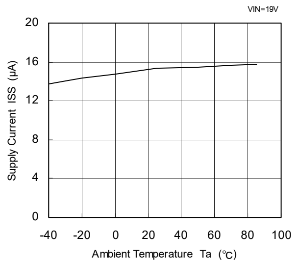
XC6202PJ02 (18V)
