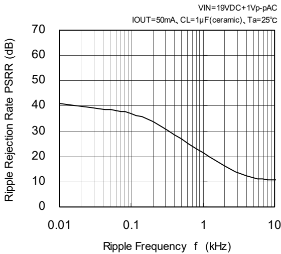
XC6202PJ02(18V)
