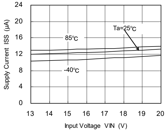
XC6202PC02(12V)
