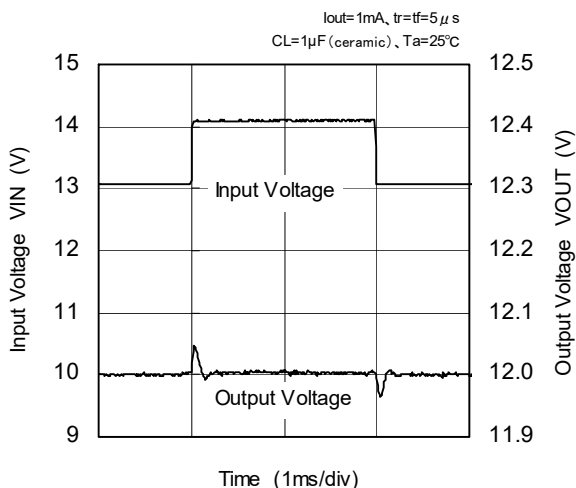
XC6202PC02 (12V)
