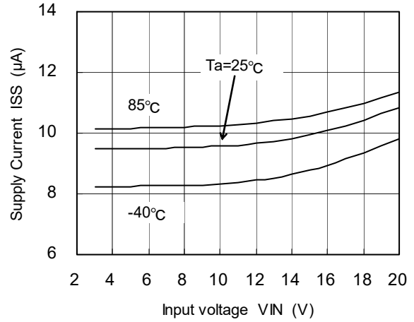
XC6202P182(1.8V)
