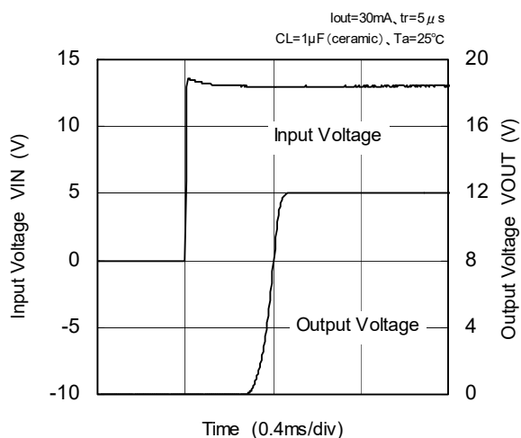
XC6202PC02 (12V)
