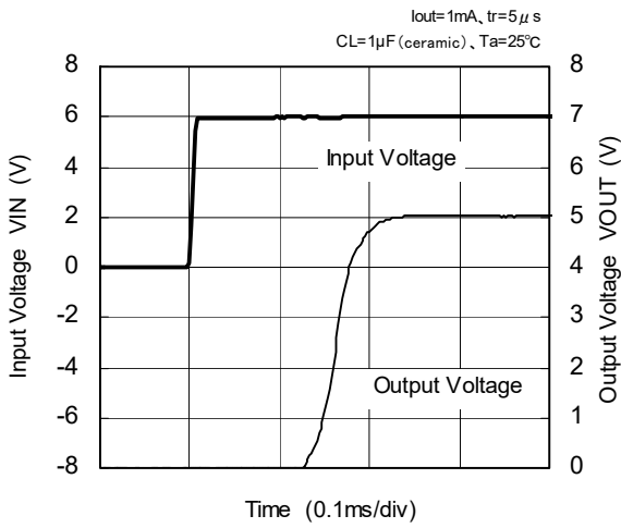
XC6202P502 (5V)
