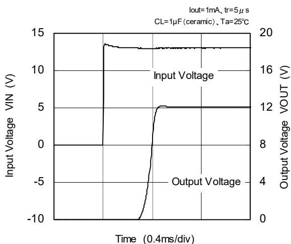
XC6202PC02 (12V)
