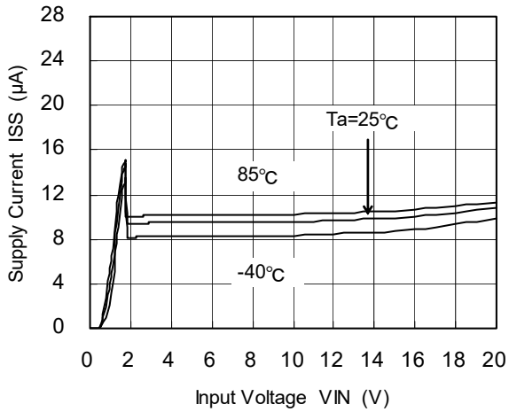
XC6202P182(1.8V)
