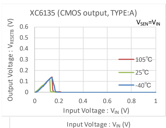
(7) Output Voltage vs. Input Voltage ( V_{IN} < \text{Operating Voltage} )
