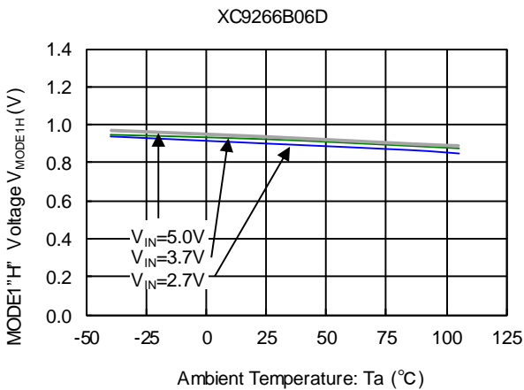
(16) MDOE1"H" Voltage vs. Ambient Temperature
