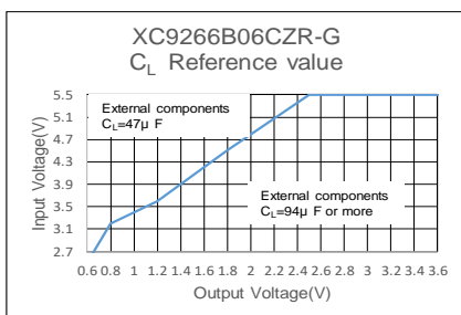
Fig.1:XC9266B06CZR-GのCL値
