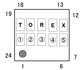
QFN0404-24C
