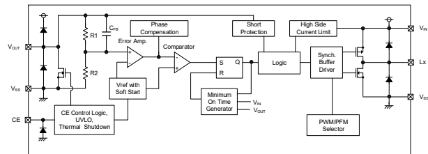
4) XC9257/XC9258 Series Type B (USP-6C)
