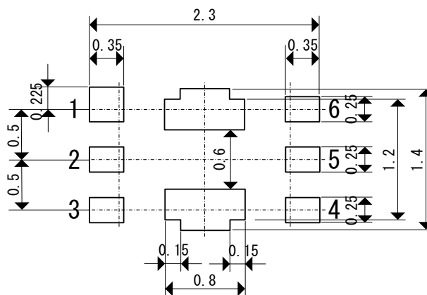
●USP-6C Reference Metal Mask Design (unit: mm) (unit: mm)
