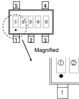
SOT-25(Under dot)
