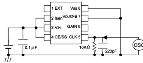
Circuit ③
