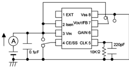
Circuit ②
