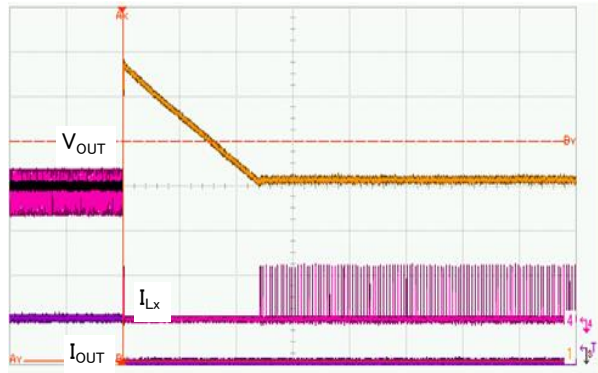
XC9136E50C(1.2MHz,PWM/PFM) V_{OUT} :100mV/div, I_{LX} :200mA/div, I_{OUT} :250mA/div, Time:1ms/div L=4.7\mu H(LTF5022-LC), C_1=20\mu F(LMK212BJ106KG*2) C_{IN}=10\mu F(LMK212BJ106KG), C_{DD}=0.47\mu F(EMK107BJ474KA)
