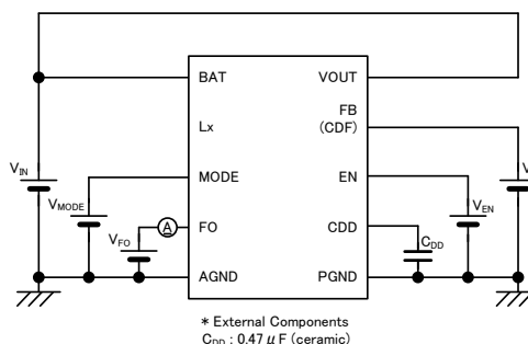
<Circuit No.7 >
