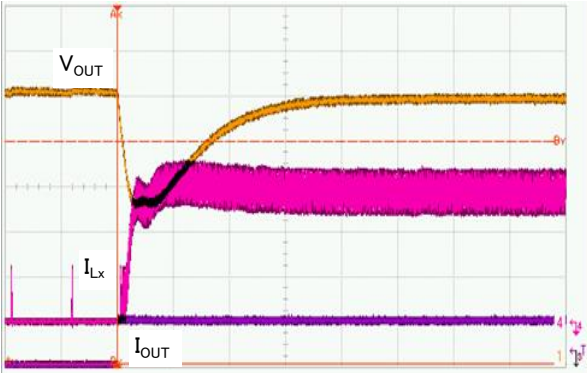
XC9136E50C(1.2MHz,PWM/PFM) V_{OUT} :100mV/div, I_{LX} :200mA/div, I_{OUT} :250mA/div, Time:50µs/div L=4.7\mu H(LTF5022-LC), C_1=20\mu F(LMK212BJ106KG*2) C_{IN}=10\mu F(LMK212BJ106KG), C_{DD}=0.47\mu F(EMK107BJ474KA)
