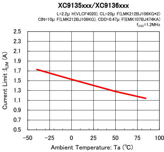
(20) Current Limit vs. Ambient Temperature
