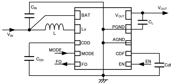
● XC9135 Series
