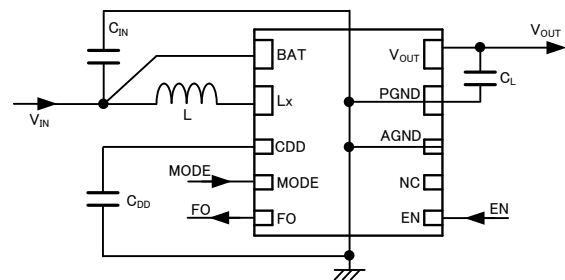
● XC9136 Series
