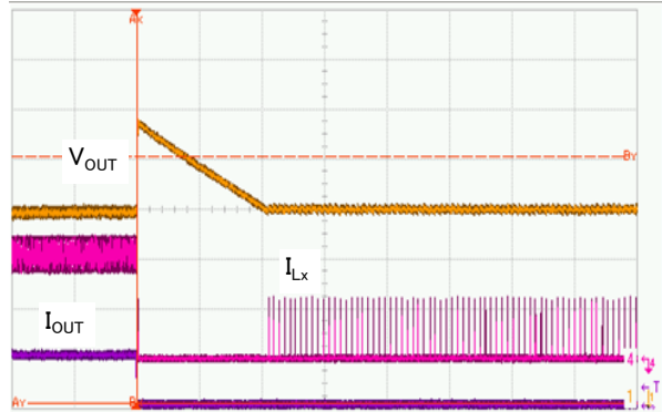
XC9136E33C (1.2MHz, PWM/PFM) V_{OUT}:100mV/div, I_{LX}:200mA/div, I_{OUT}:200mA/div, Time:1ms/div L=4.7\mu H(LTF5022-LC), C_L=20\mu F(LMK212BJ106KG*2) C_{IN}=10\mu F(LMK212BJ106KG), C_{DD}=0.47\mu F(EMK107BJ474KA)
