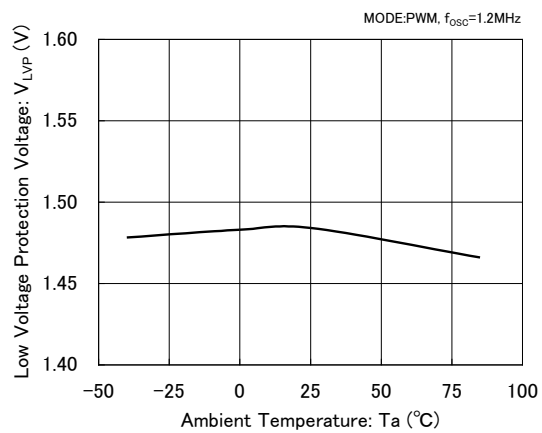
XC9135K
