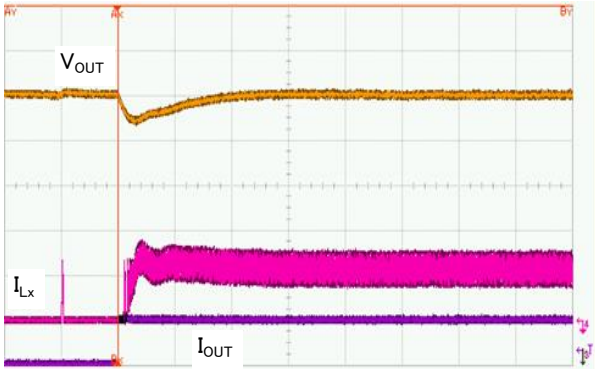
XC9136E18C (1.2MHz, PWM/PFM) V_{OUT}:100mV/div, I_{LX}:200mA/div, I_{OUT}:50mA/div, Time:50\mu s/div L=2.2\mu H(LTF5022-LC), C_L=20\mu F(LMK212BJ106KG*2) C_{IN}=10\mu F(LMK212BJ106KG), C_{DD}=0.47\mu F(EMK107BJ474KA)
