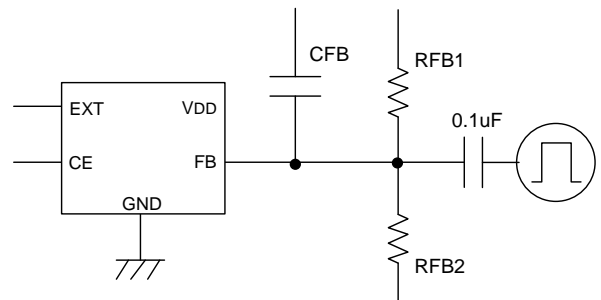
Circuit ⑥
