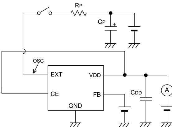
Circuit ④
