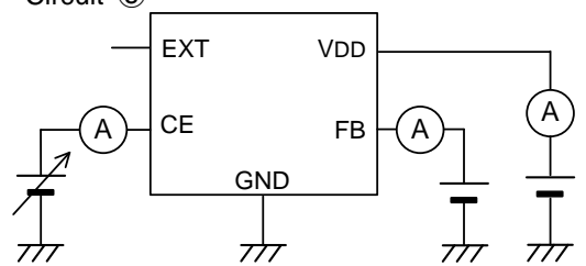
Circuit ⑤
