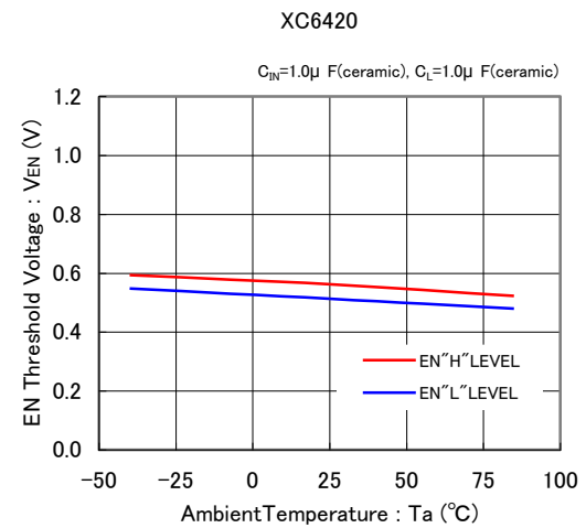
(7) EN Threshold Voltage vs. AmbientTemperature
