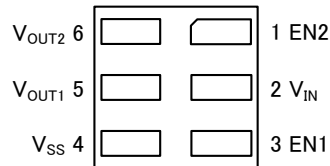
USPN-6 (BOTTOM VIEW)
