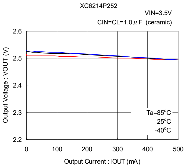
(1) Output Voltage vs. Output Current (Continued)
