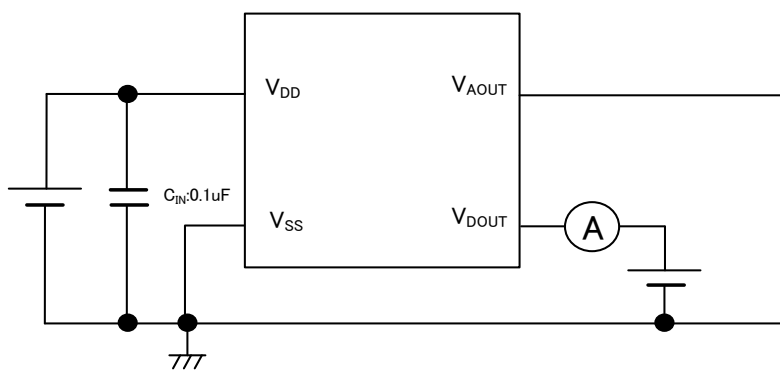
Circuit ③
