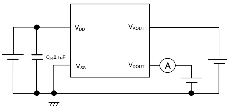
Circuit ④
