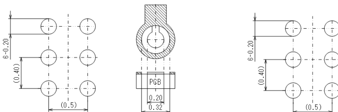
WLP-6-05 Reference Pattern Layout
