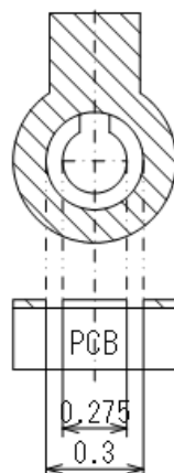
WLP-5-03 Reference Pattern Layout detail
