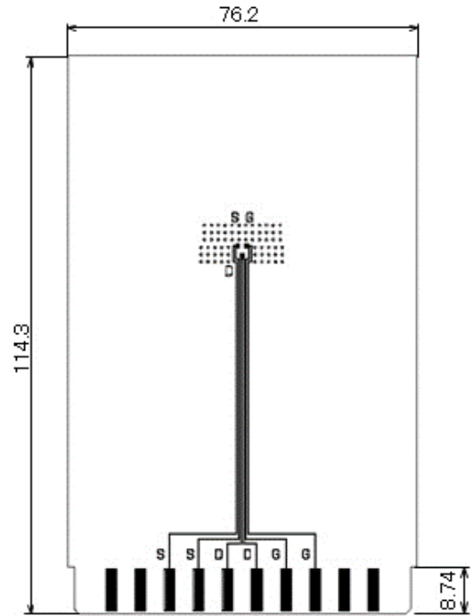
Evaluation Board (Unit: mm)
