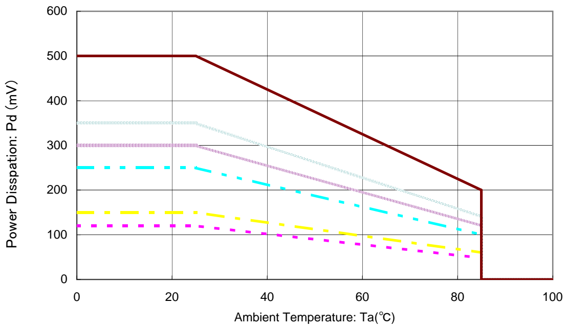
Package Power Dissipation vs. Ambient Temperature
